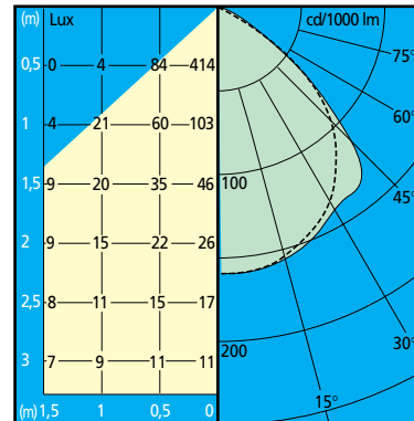
PLDE109 prisma — C = 0 of 180° --- C = 90 of 270°
